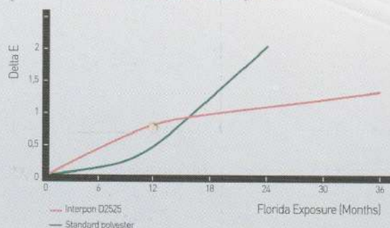
2. Color Retention Graph
