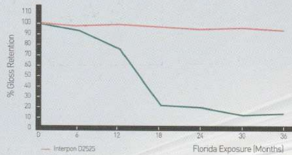
1. Gloss Retention Graph
